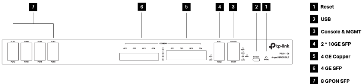
Front View of P1201-08
